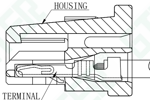
ASSEMBLY LAYOUT
