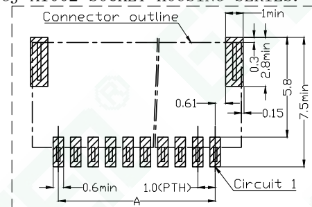
SMT SIDE ENTRY TYPE PCB LAYOUT
