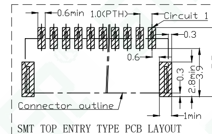
SMT TOP ENTRY TYPE PCB LAYOUT
