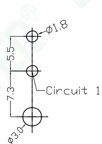
2x01P PCB LAYOUT
