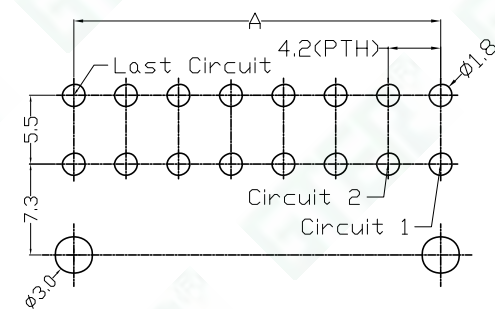
2x03P-2x12P PCB LAYOUT
